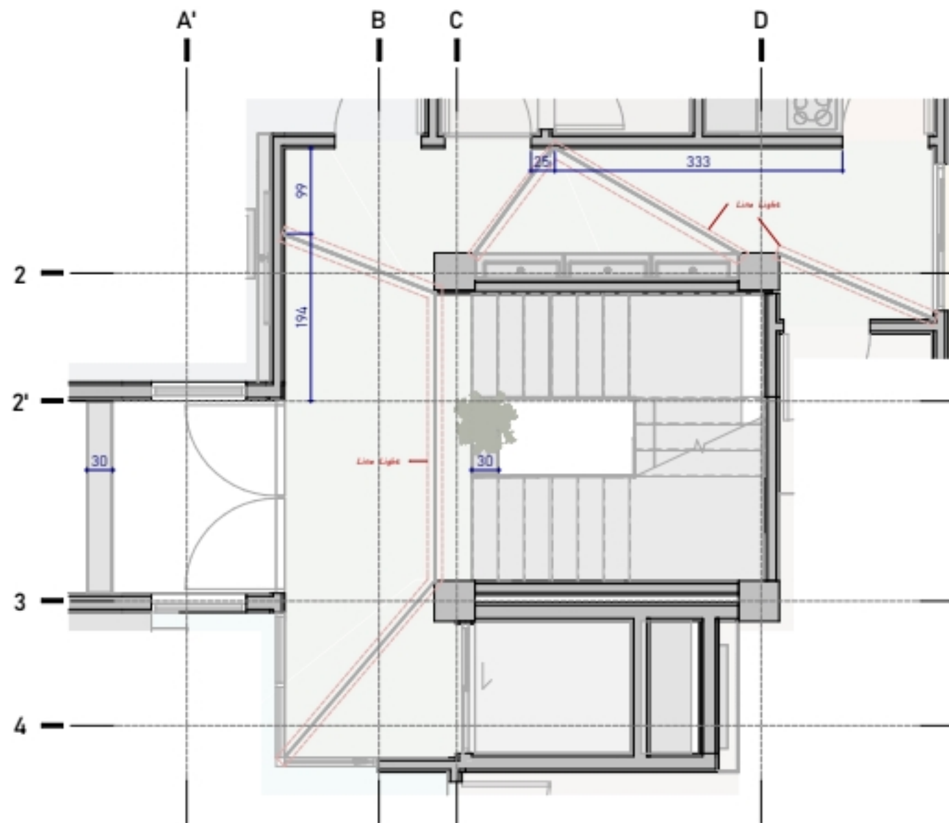
1. SECOND-CORRIDOR-LAYOUT18
