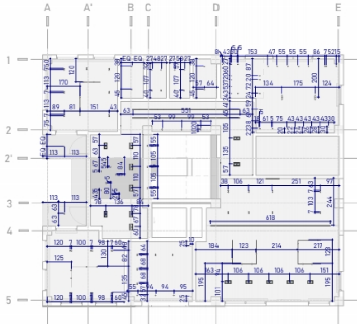
1. FIRST CEILING LIGHTING DIM PLAN
