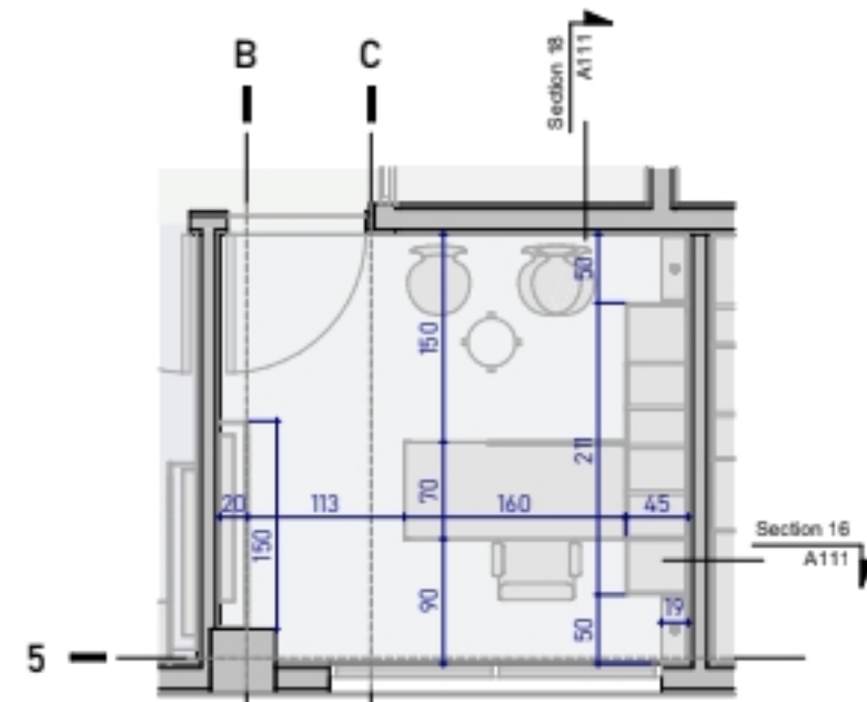
3. FIRST - LAYOUT 07
