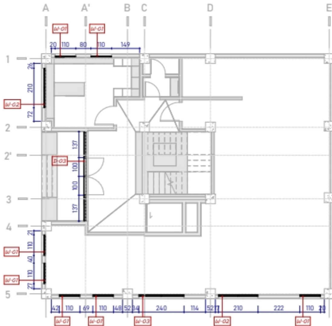
1. Window Dimension Plan-GF
