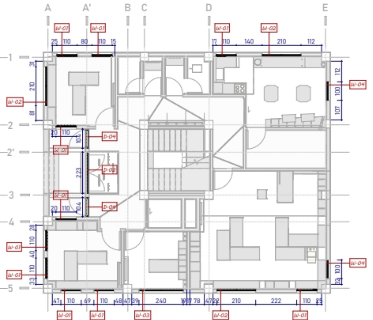
2. Window Dimension Plan _ 1st
