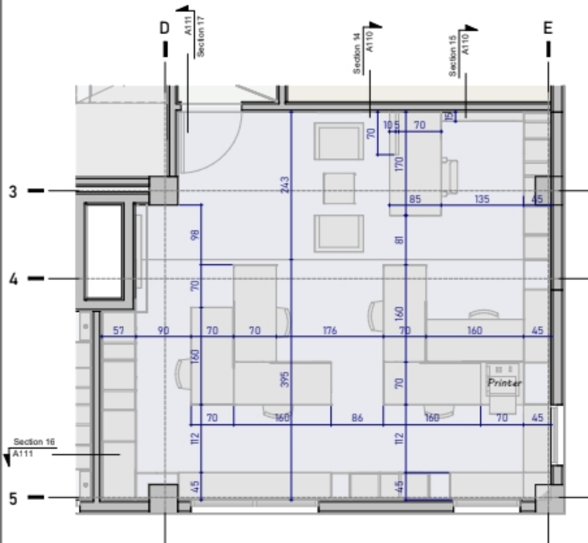
1. FIRST -FINANCIAL ROOM-LAYOUT 06
