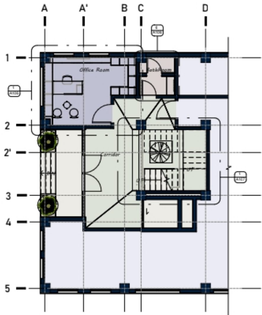
1. G.F-LAYOUT HOT KEY PLAN
