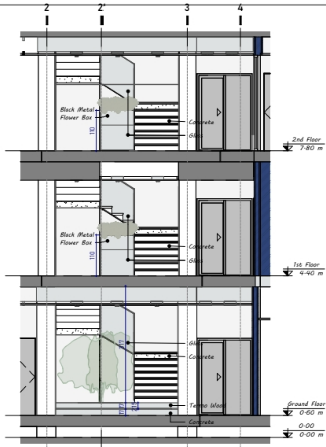
2. SECTION 5
