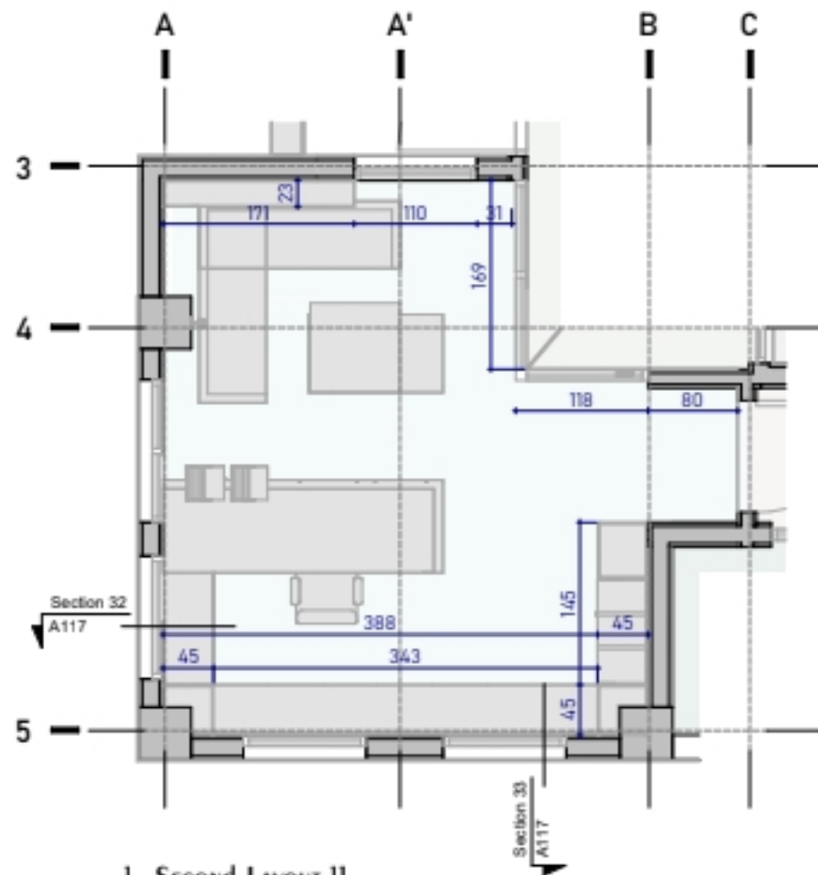
1. Second-Layout II
