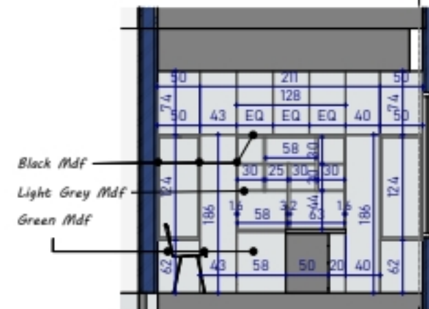
4. SECTION 18
