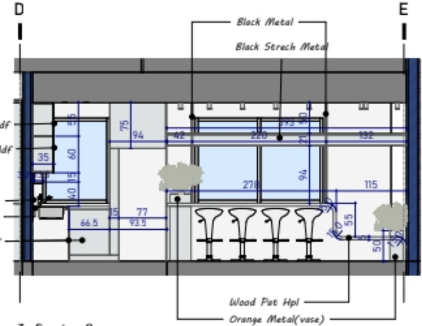
3. SECTION 9
