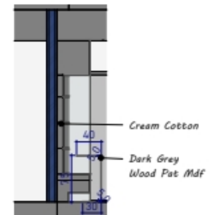
7. SECTION 13
