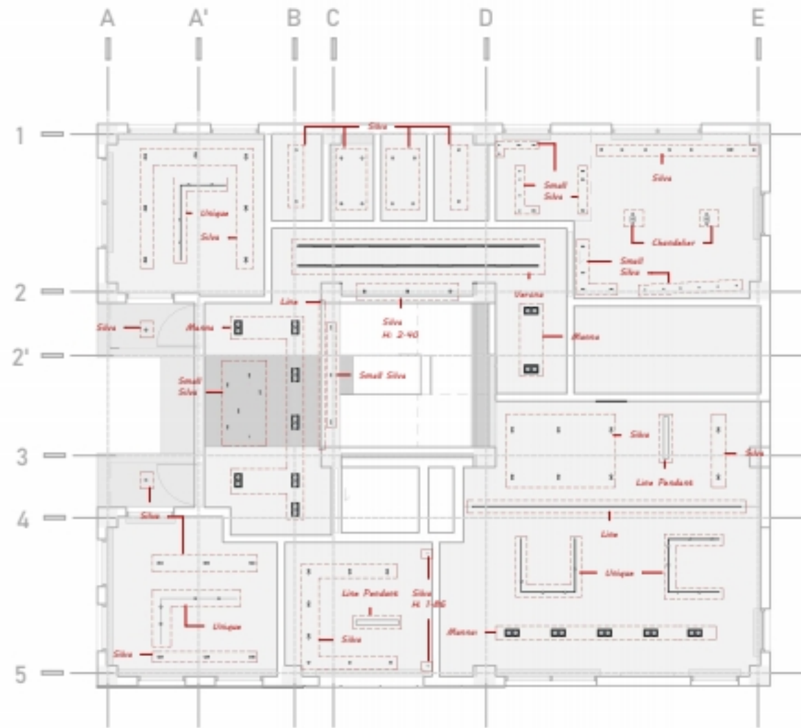
1. FIRST CEILING LIGHTING PLAN
