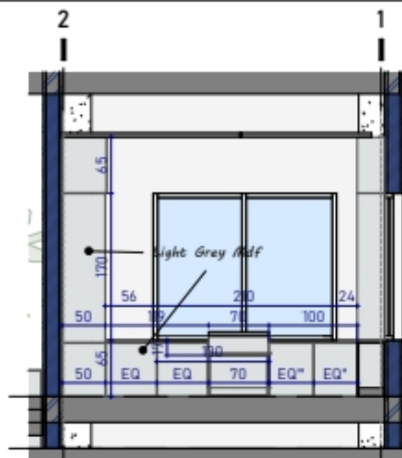
2. SECTION 1
