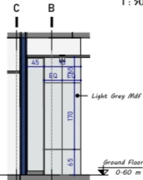
5. SECTION 4
