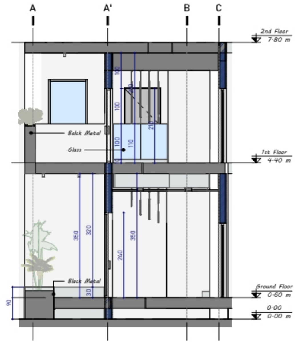
2. SECTION 26
