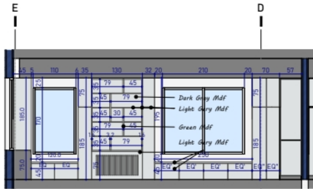
1. SECTION 16
