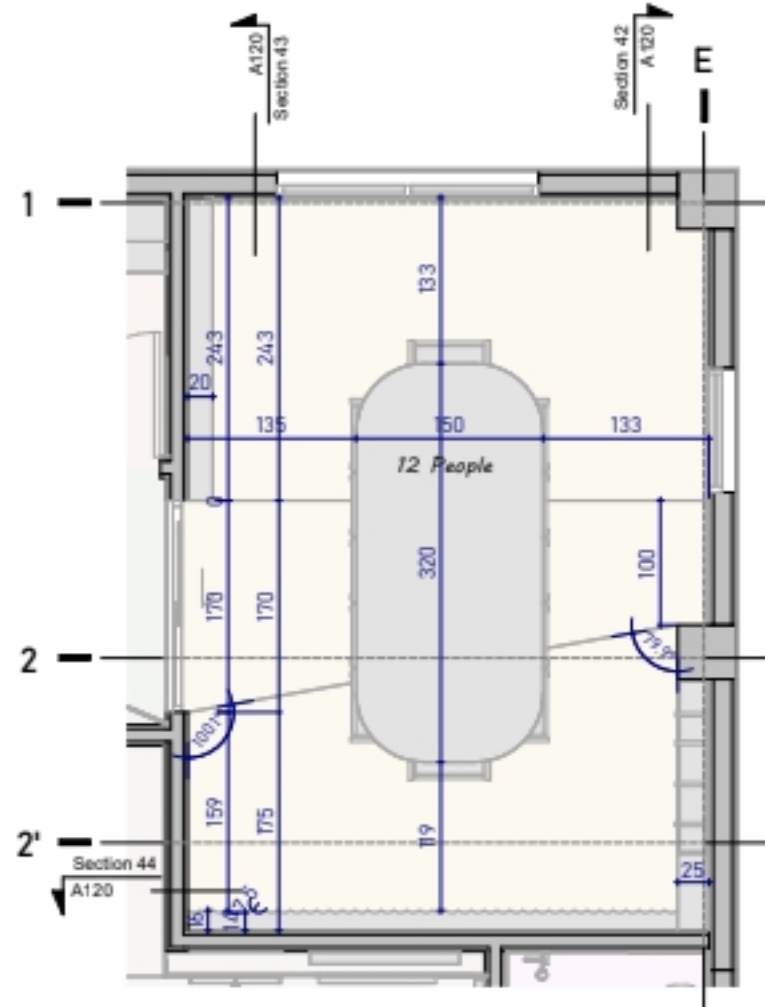
1. SECOND-CONFERENCE ROOM-LAYOUT 14
