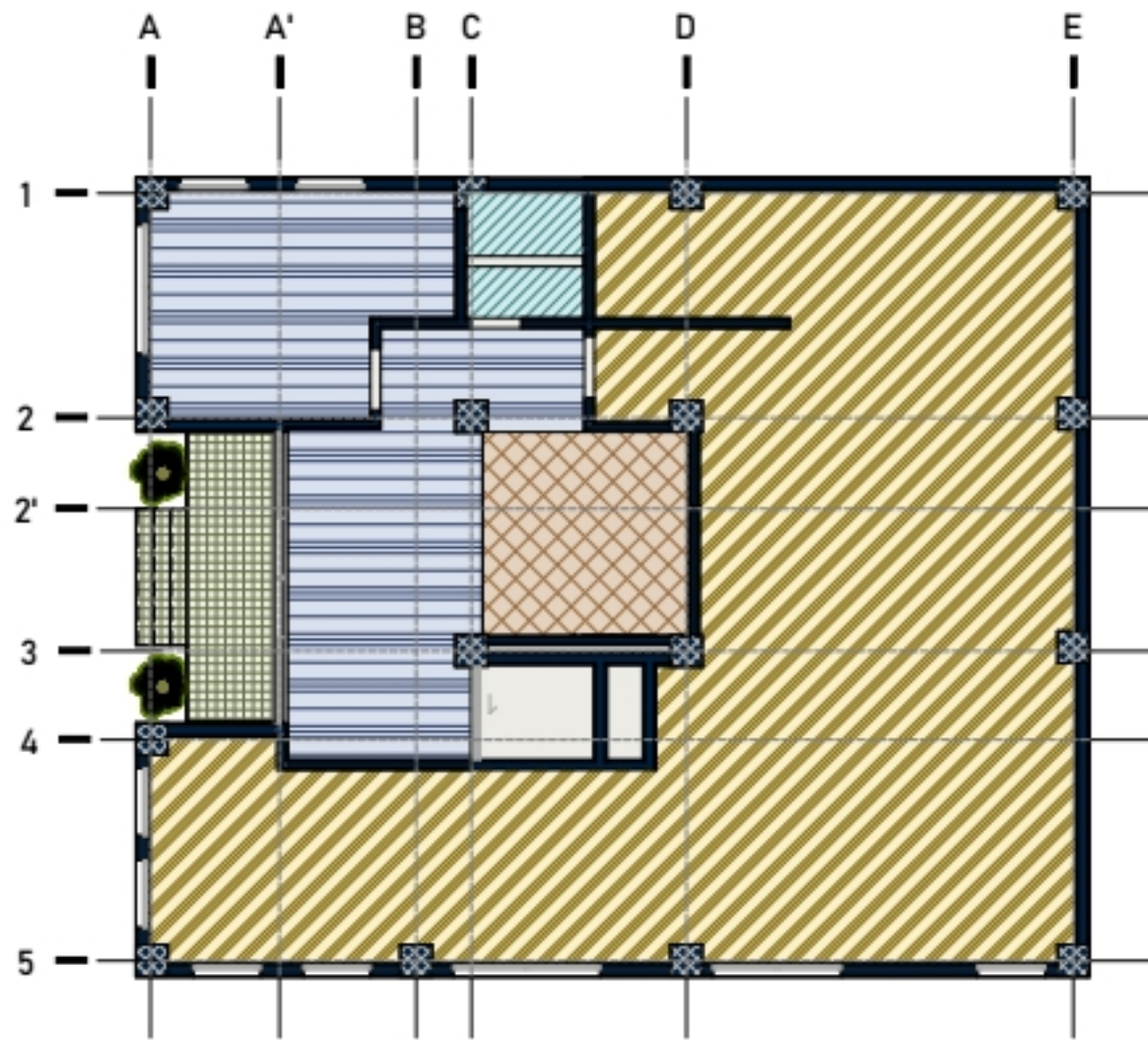
1. GROUND FLOOR-FLOORING PLAN
