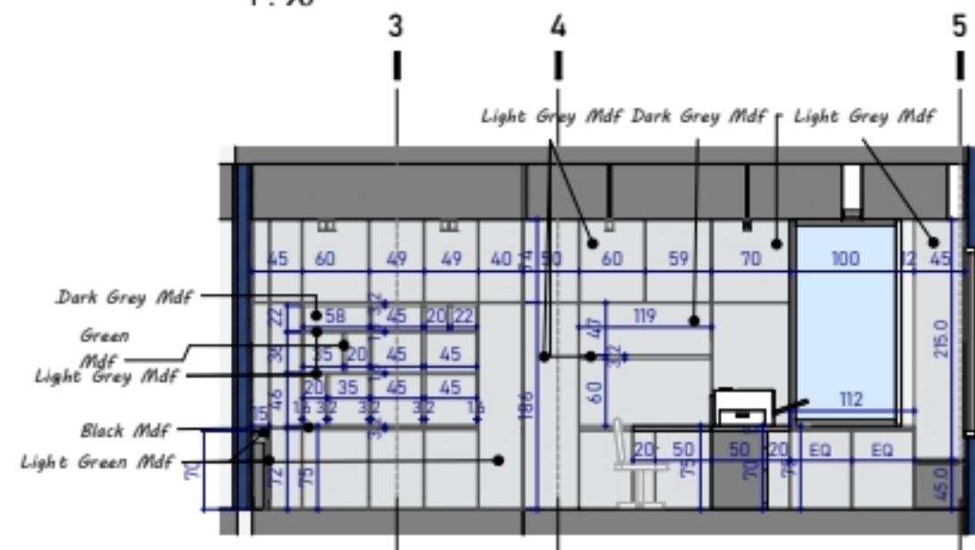
3. SECTION 15
