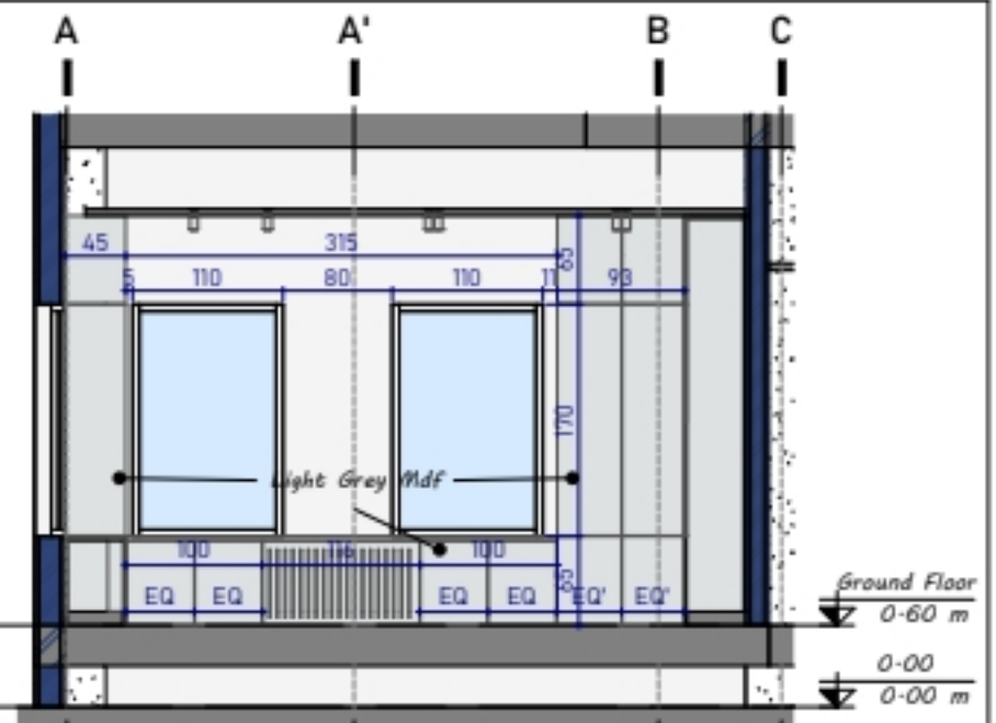
3. SECTION 2
