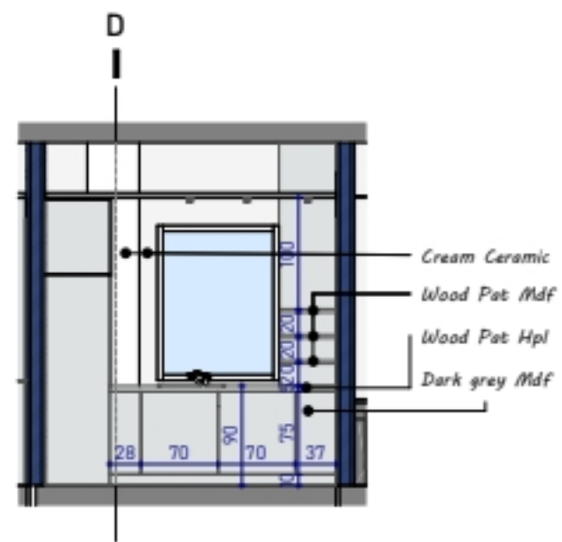
3. SECTION 46
