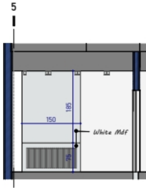
2. SECTION 20
