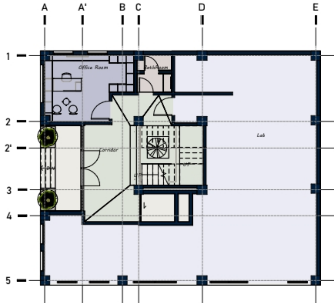
1.1-GROUND FLOOR_FURNITURE PLAN
