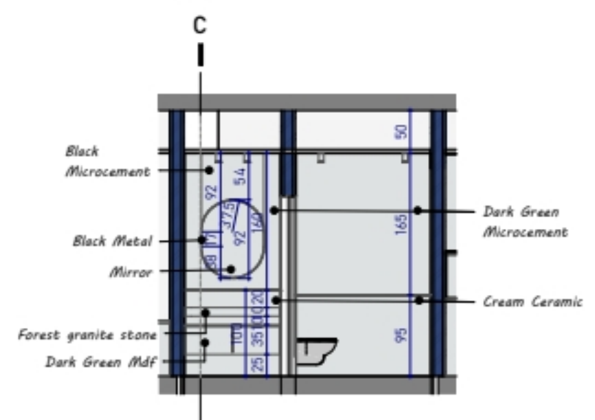
6. SECTION 48
