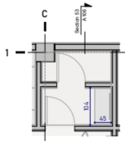
6. Gf-LAYOUT BATHROOM
