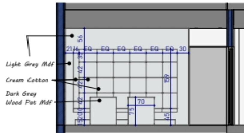
6. SECTION 12
