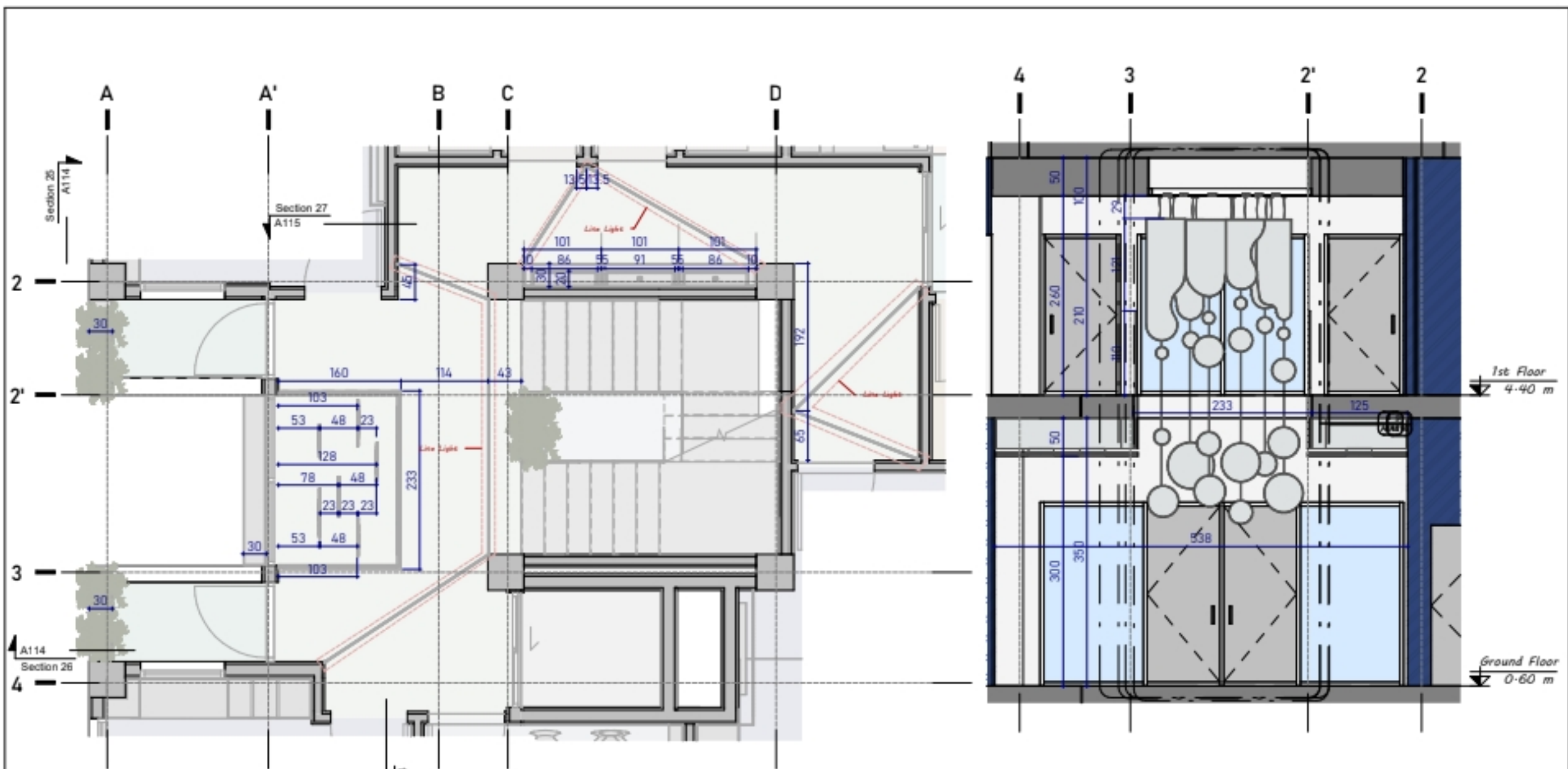
1. FIRST-CORRIDOR-LAYOUT 09 1 : 50
