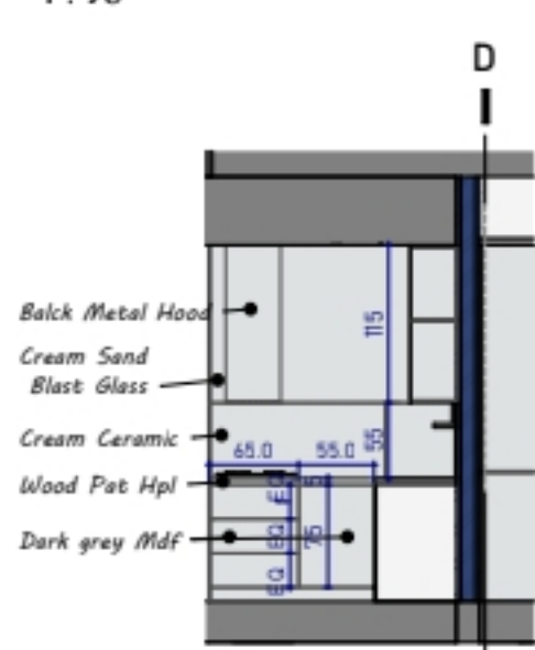
4. SECTION 10
