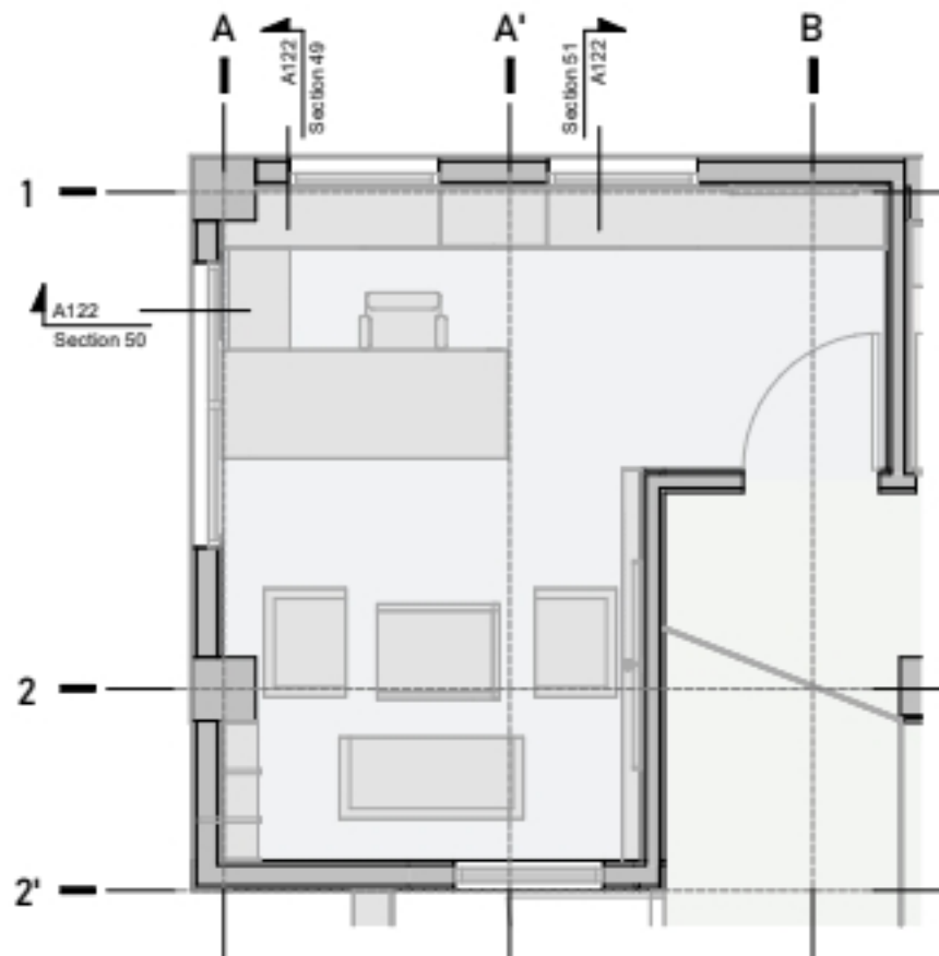
1. SECOND-MANAGER OFFICE-LAYOUT I7 1 : 50
