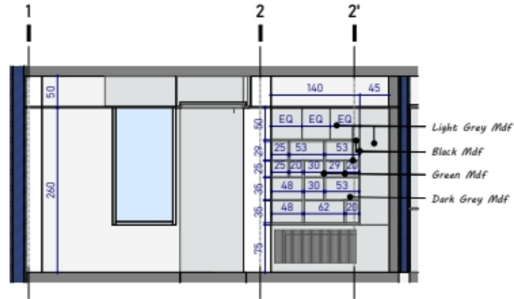
2. SECTION 42
