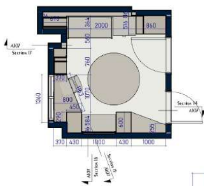
1. Bedroom Layout
