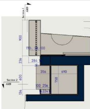
1. ENTRANCE LAYOUT 1 : 25
