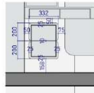
6. DRAWER LAYOUT 1 : 20
