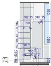
5. MIRROR LAYOUT 1 : 50
