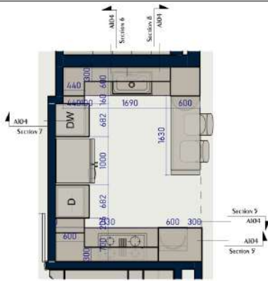
1. KITCHEN LAYOUT
